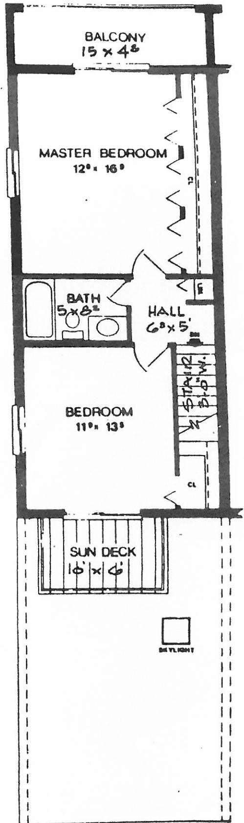
SECOND FLOOR
